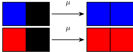
Reproduction
