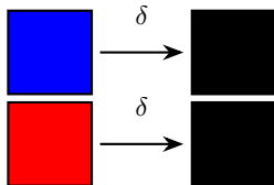
Death
