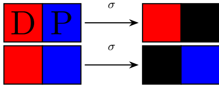
Selection
