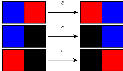
Exchange
